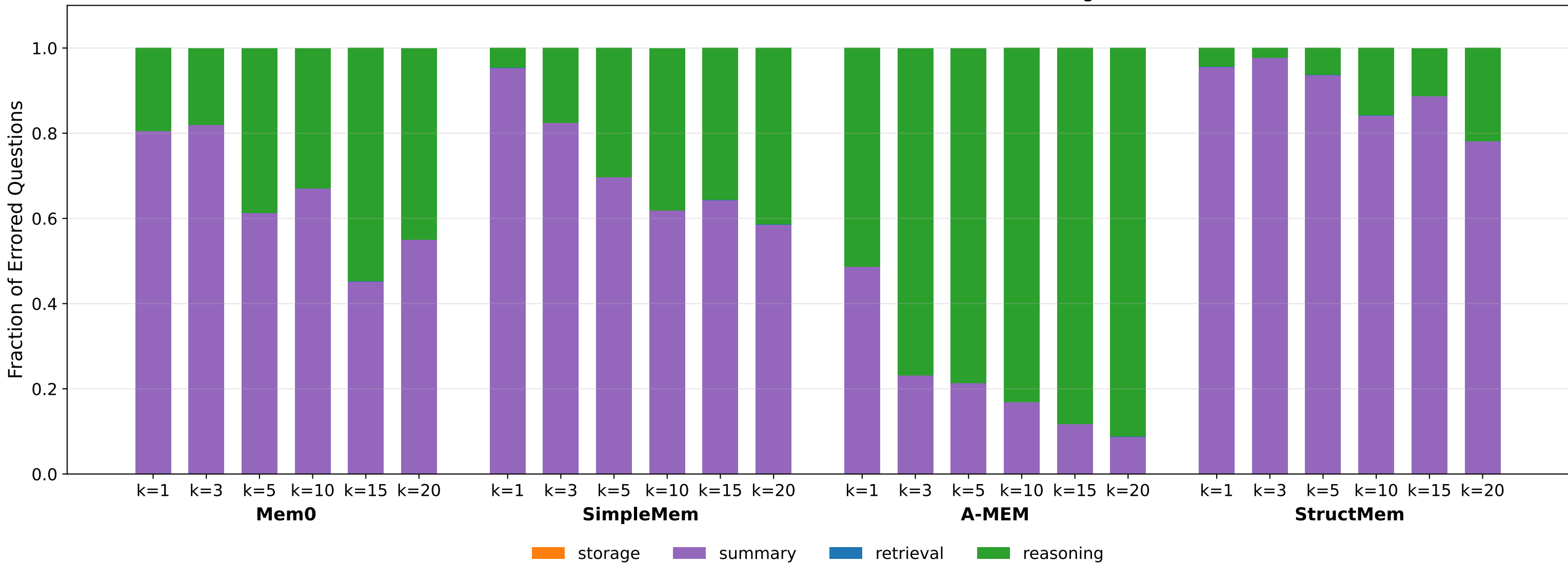
Error breakdown vs. k — Persona-Retrieval (Misleading)
