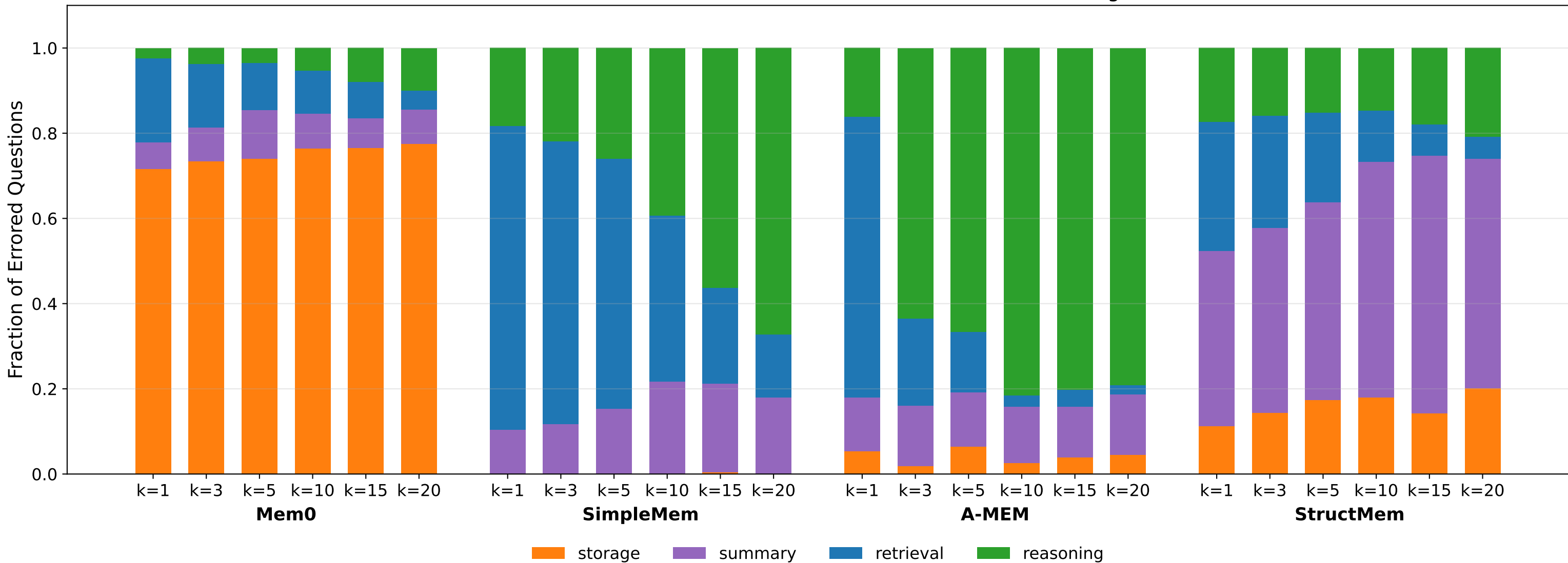
Error breakdown vs. k — Persona-Retrieval (Non-misleading)
