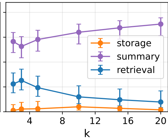
StructMem
