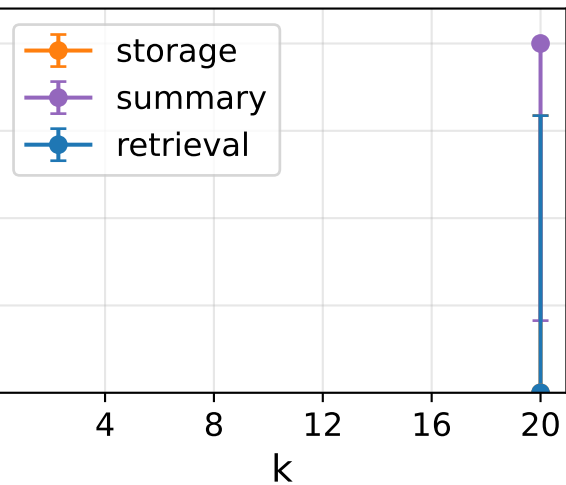
StructMem
