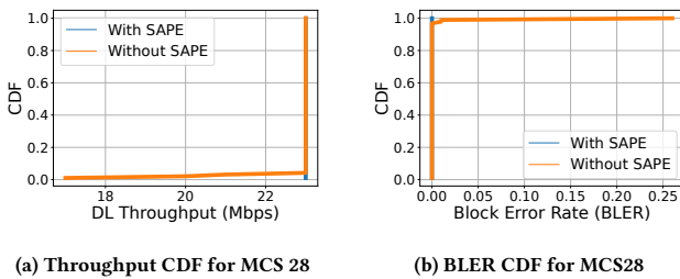
Figure 7: Indoor LOS (Clean) Results.
