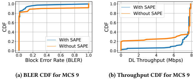
Figure 6: Indoor NLOS (Heavy Multipath) - POS2 Results.
