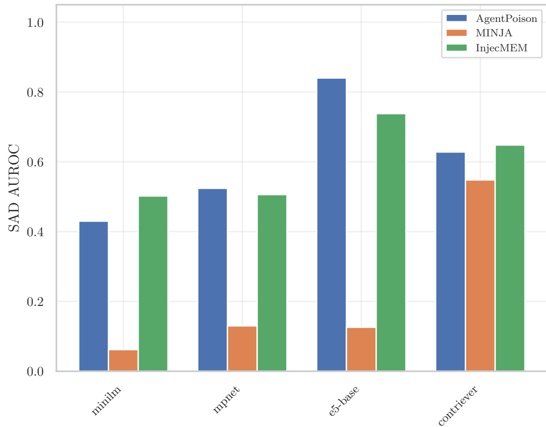
Cross-Encoder SAD AUROC
