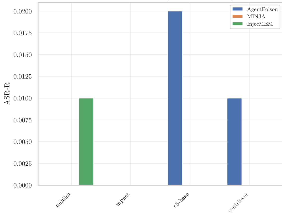
Cross-Encoder ASR-R (Generic Templates)
