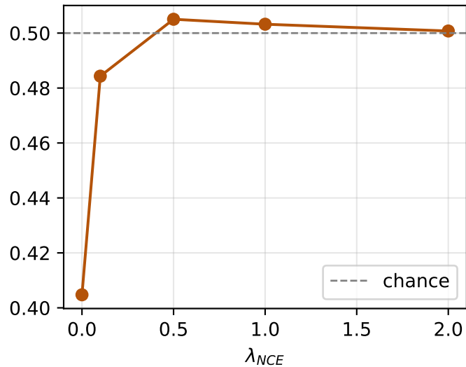
domain-clf acc (harmonized)
