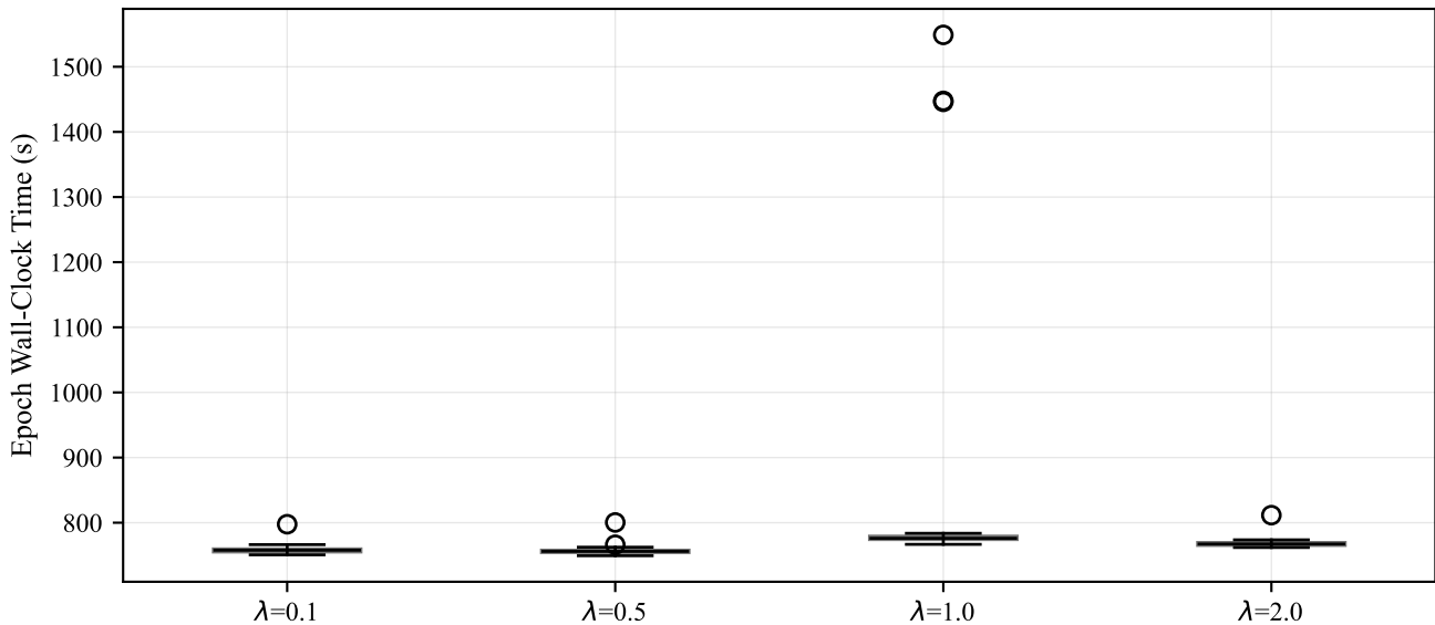
Per-Epoch Wall-Clock Time on NVIDIA A100-PCIE
