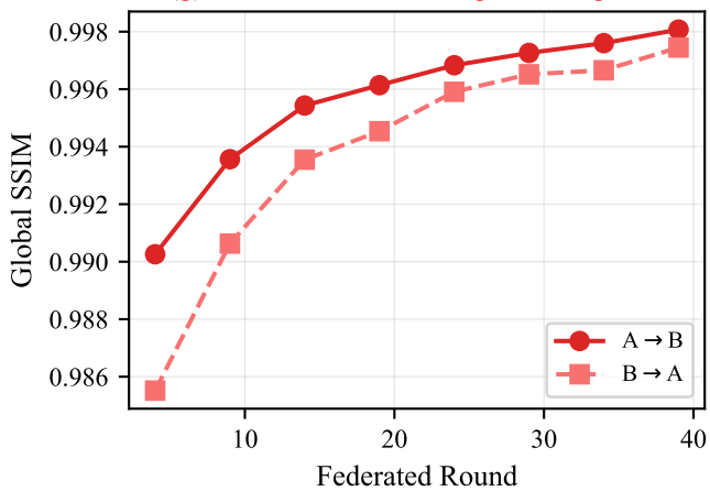
(g) Extension E: FedAvg Convergence
