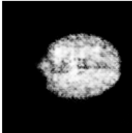
harmonized T1
