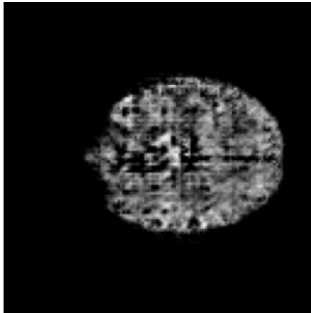
harmonized FLAIR
