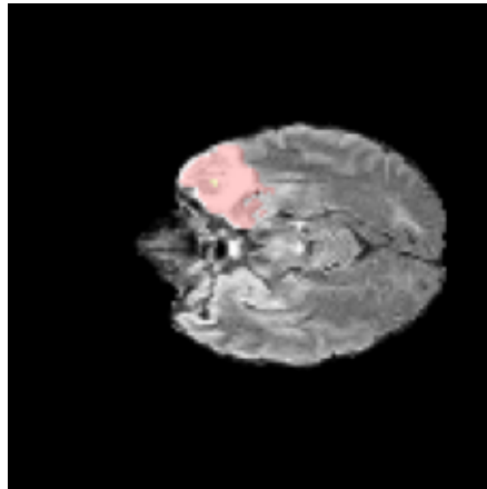
tumor (GT)
