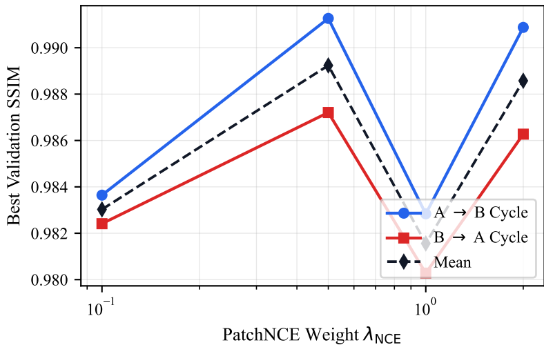
SSIM vs \lambda_{\text{NCE}}
