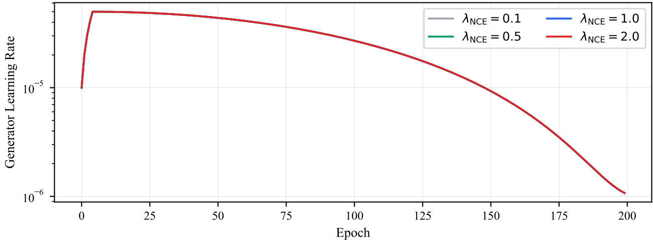
Cosine Annealing with Linear Warmup ( \eta_0 = 5 \times 10^{-5} )
