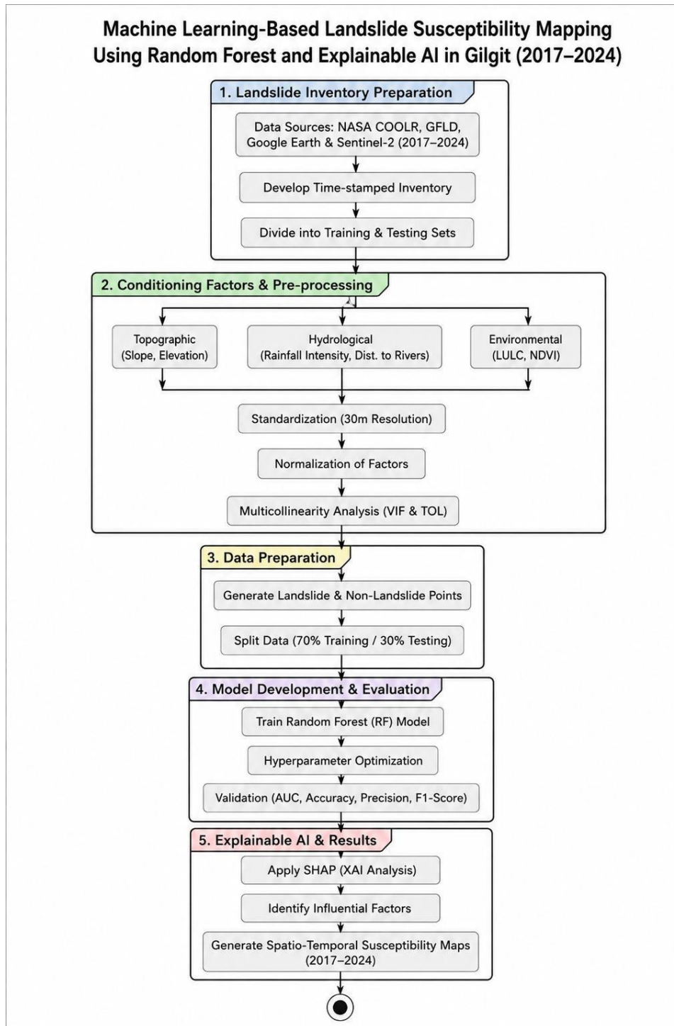
Figure 2: Methodological Framework for Landslide Susceptibility Mapping Using Random Forest and Explainable AI
