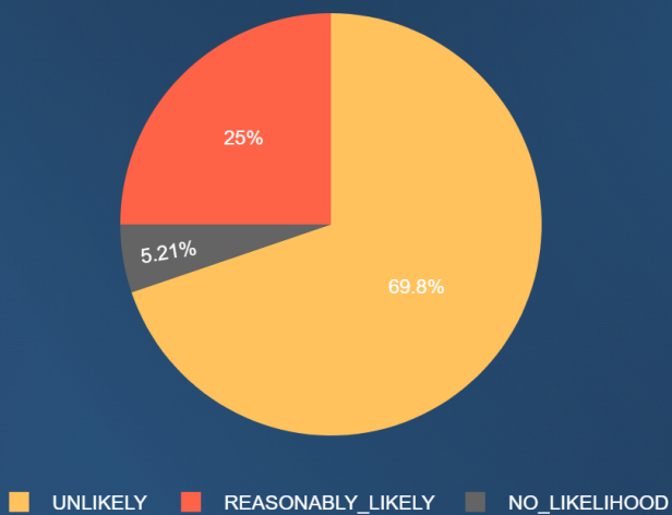
Likelihood Distribution
