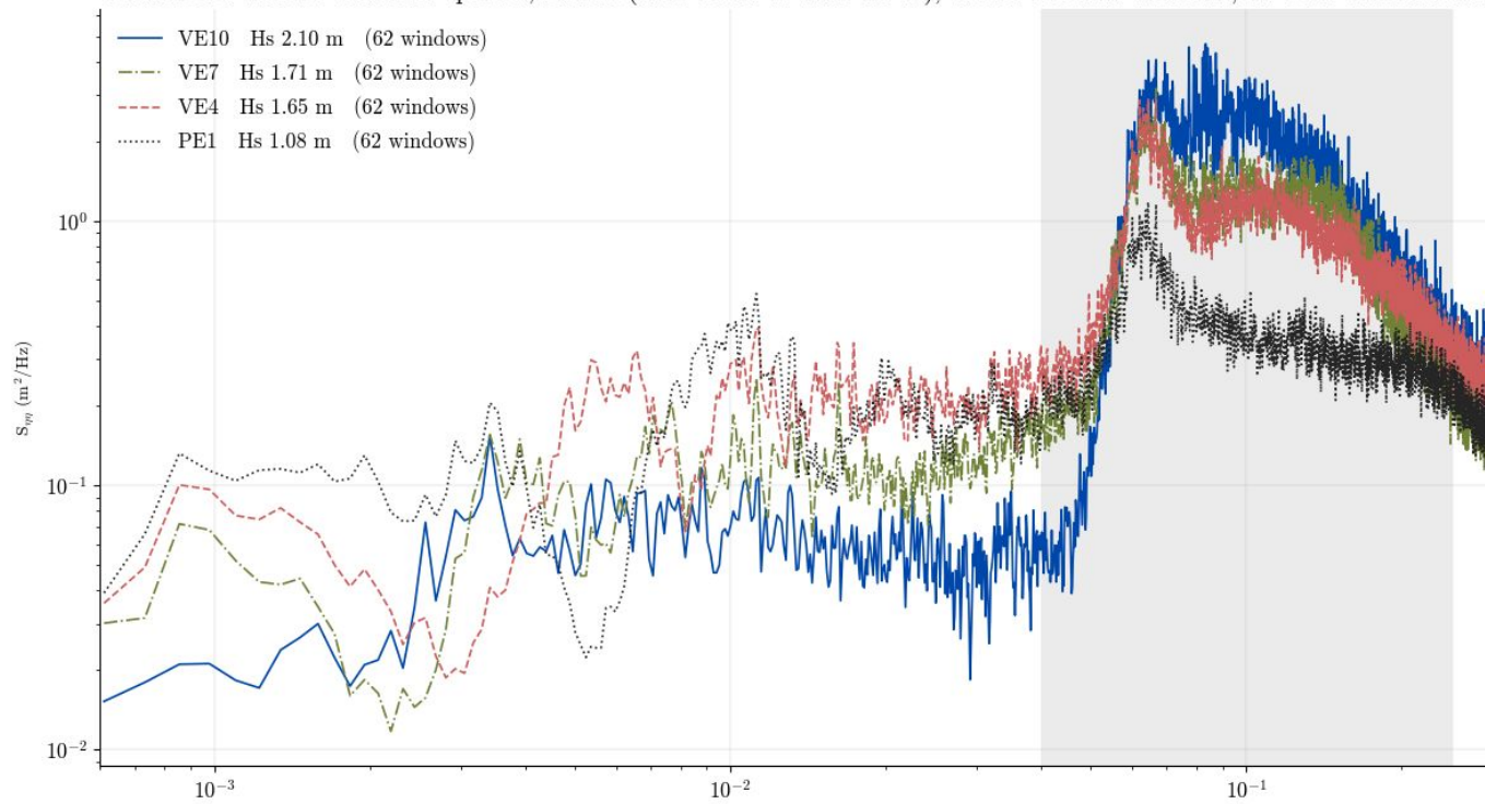
Transect E: surface elevation spectra, Lowell (2026-09-07 to 2026-09-09), Welch 137 min windows, Hs over 0.04-0.25 Hz
