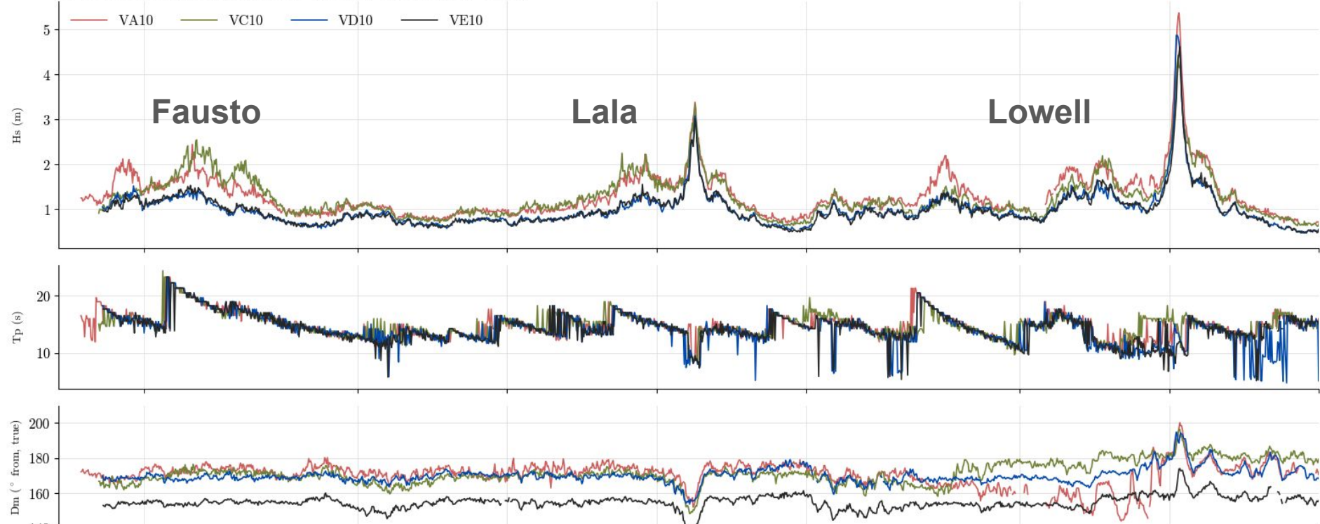
10 m sensors: Hs, Tp, Dm (0.04-0.25 Hz, 1h averages, UTC)
