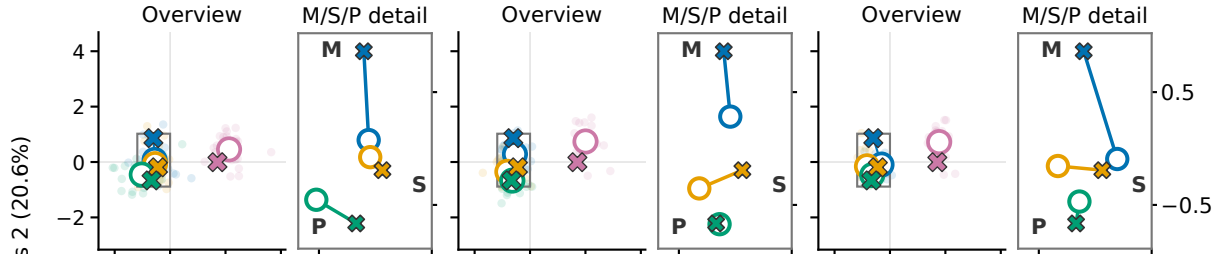
GPT Image 1
