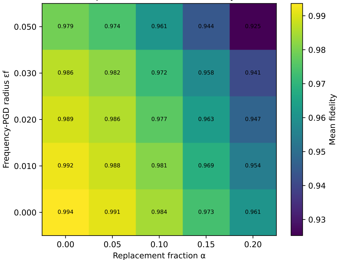
1-qubit combined-attack fidelity
