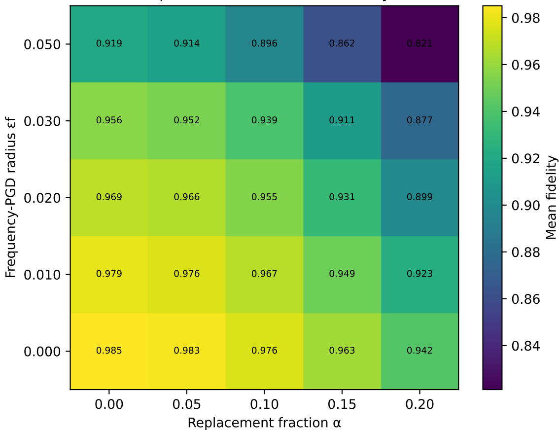
2-qubit combined-attack fidelity
