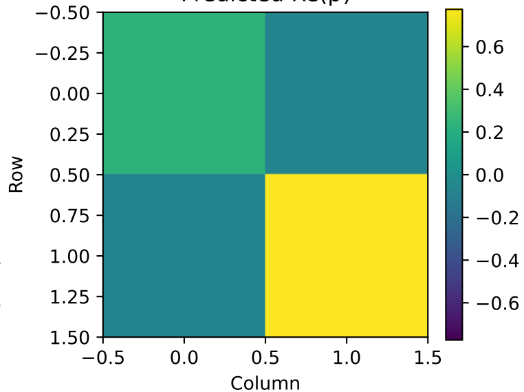
Predicted \text{Re}(\hat{\rho})
