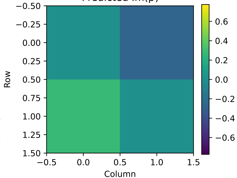
Predicted \text{Im}(\hat{\rho})
