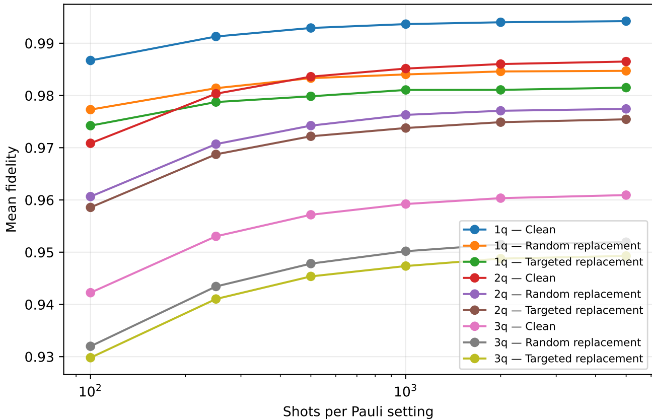
Shot-noise sensitivity
