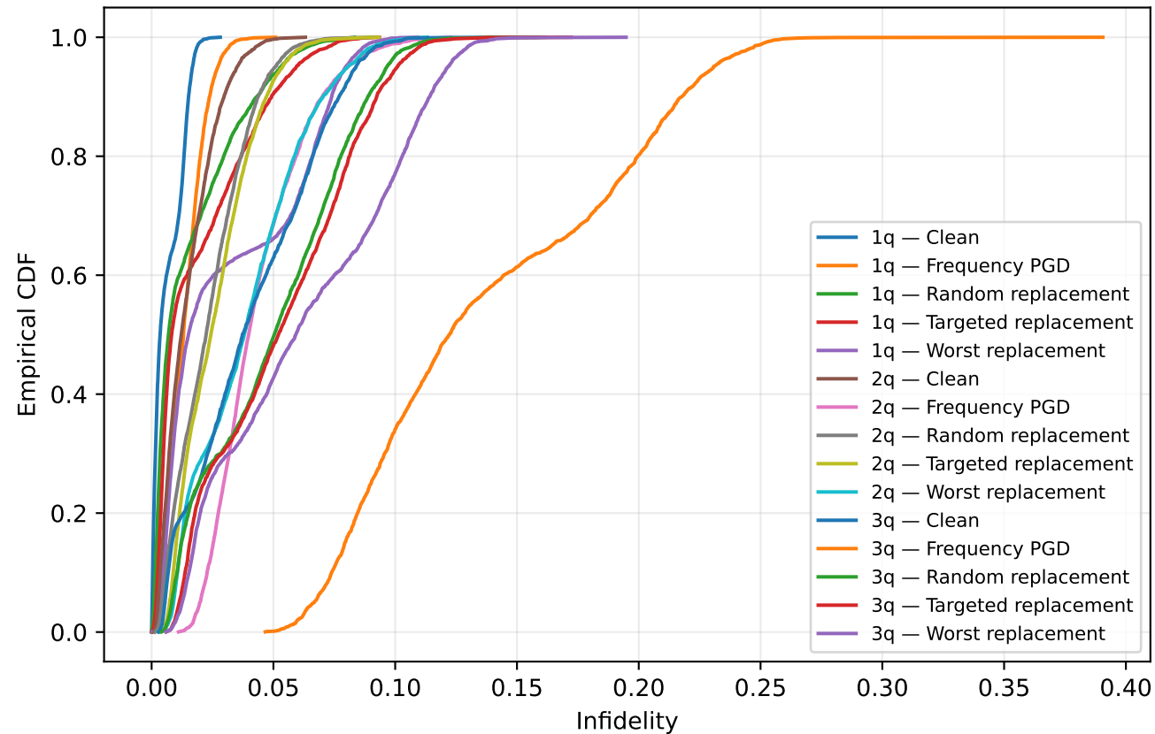
Infidelity distribution
