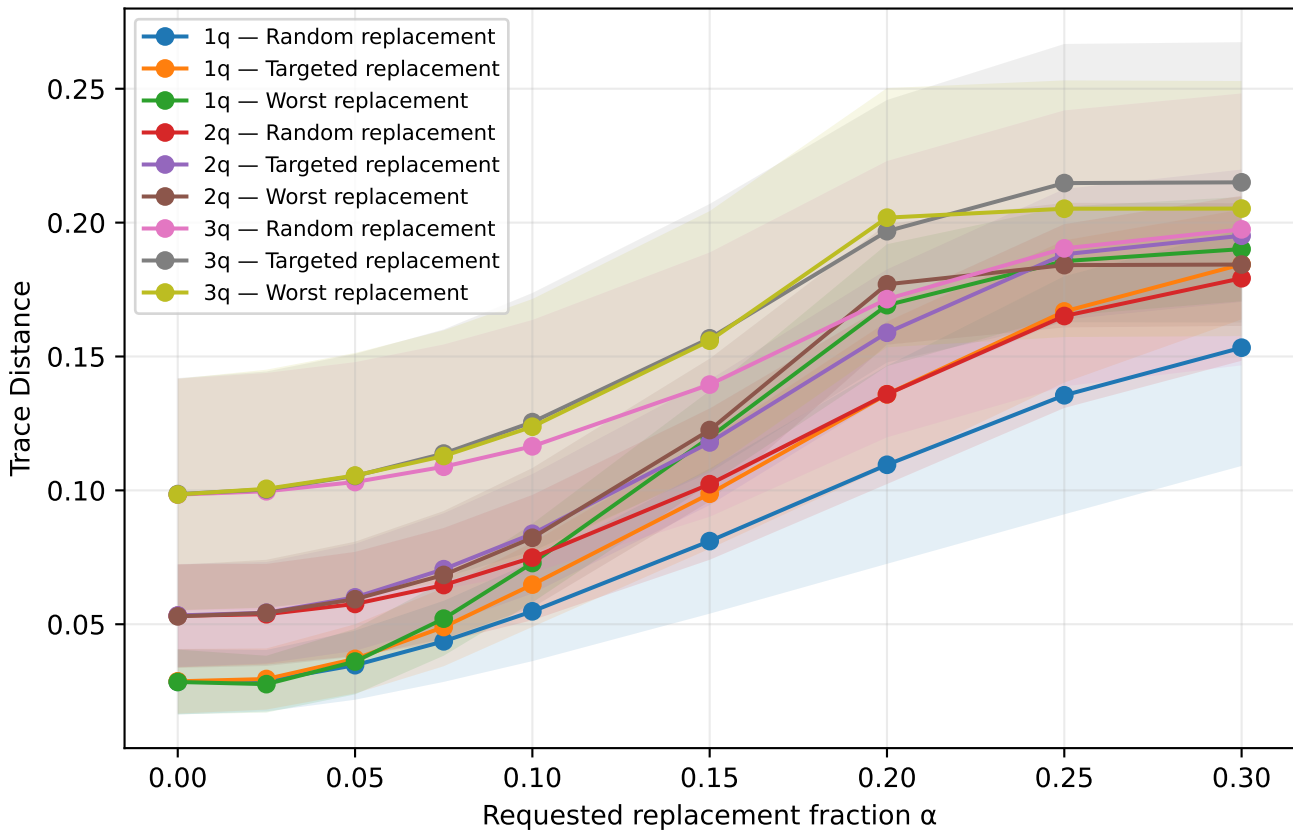
Trace Distance versus replacement fraction
