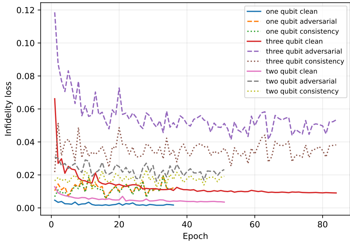
Validation loss components
