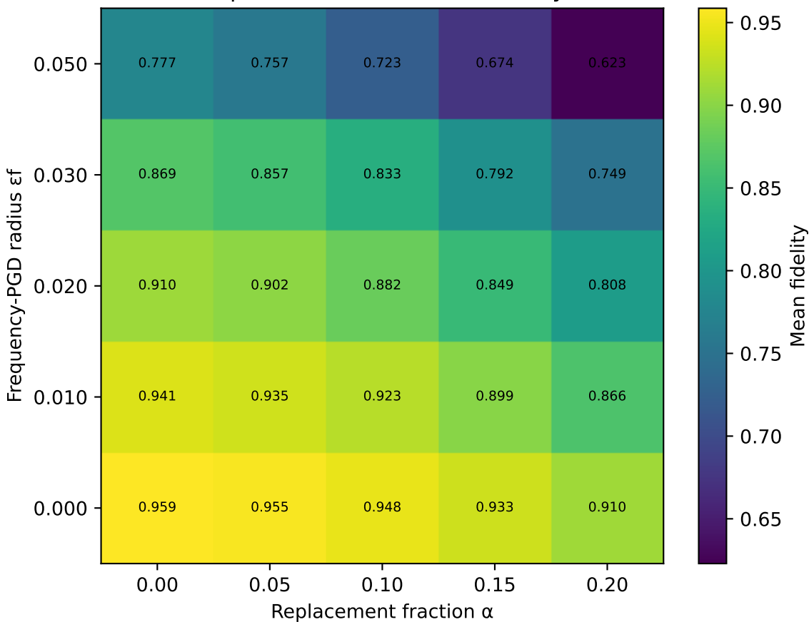
3-qubit combined-attack fidelity
