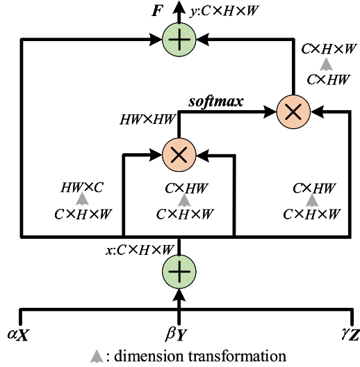
Fig. 5. Architecture of the proposed multihead cosine nonlocal attention module. \oplus denotes the elementwise addition and \otimes denotes the matrix multiplication.
