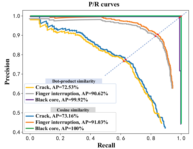
Fig. 10. P/R curves of different similarity calculation methods for three types of defects.
