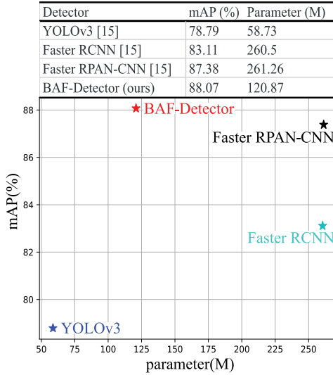
Fig. 4. Comparison of BAF-Detector with Su et al. [15].
