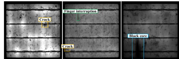
Fig. 2. Three raw EL near-infrared images with two crack defects in yellow boxes, one finger interruption defect in green box, and one black core defect in blue box.
