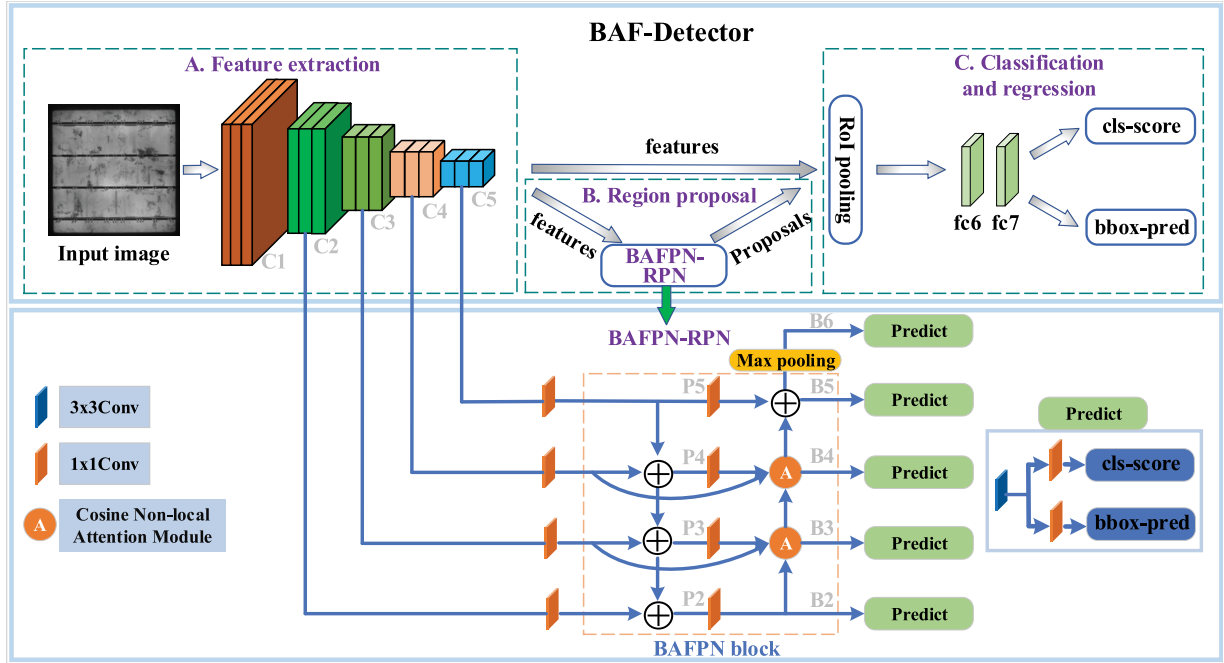
Fig. 8. Architecture of the proposed BAFPN detector (BAF-Detector).
