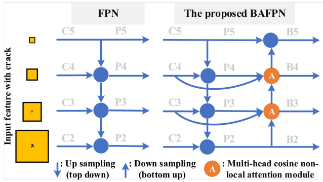
Fig. 3. Architecture of FPN and the proposed bidirectional attention FPN (BAFPN).
