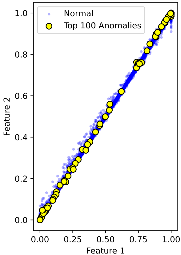
Feature Space with Anomalies
