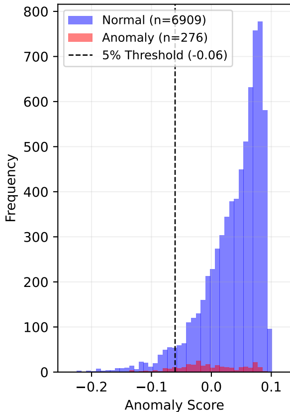
Distribution of Anomaly Scores
