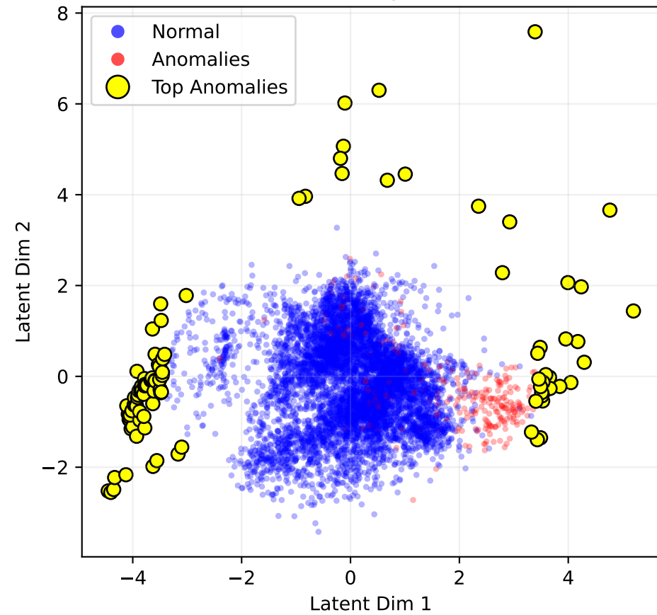
Latent Space
