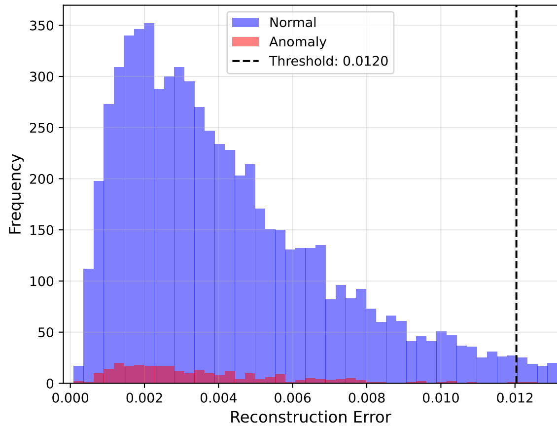
Reconstruction Error Distribution
