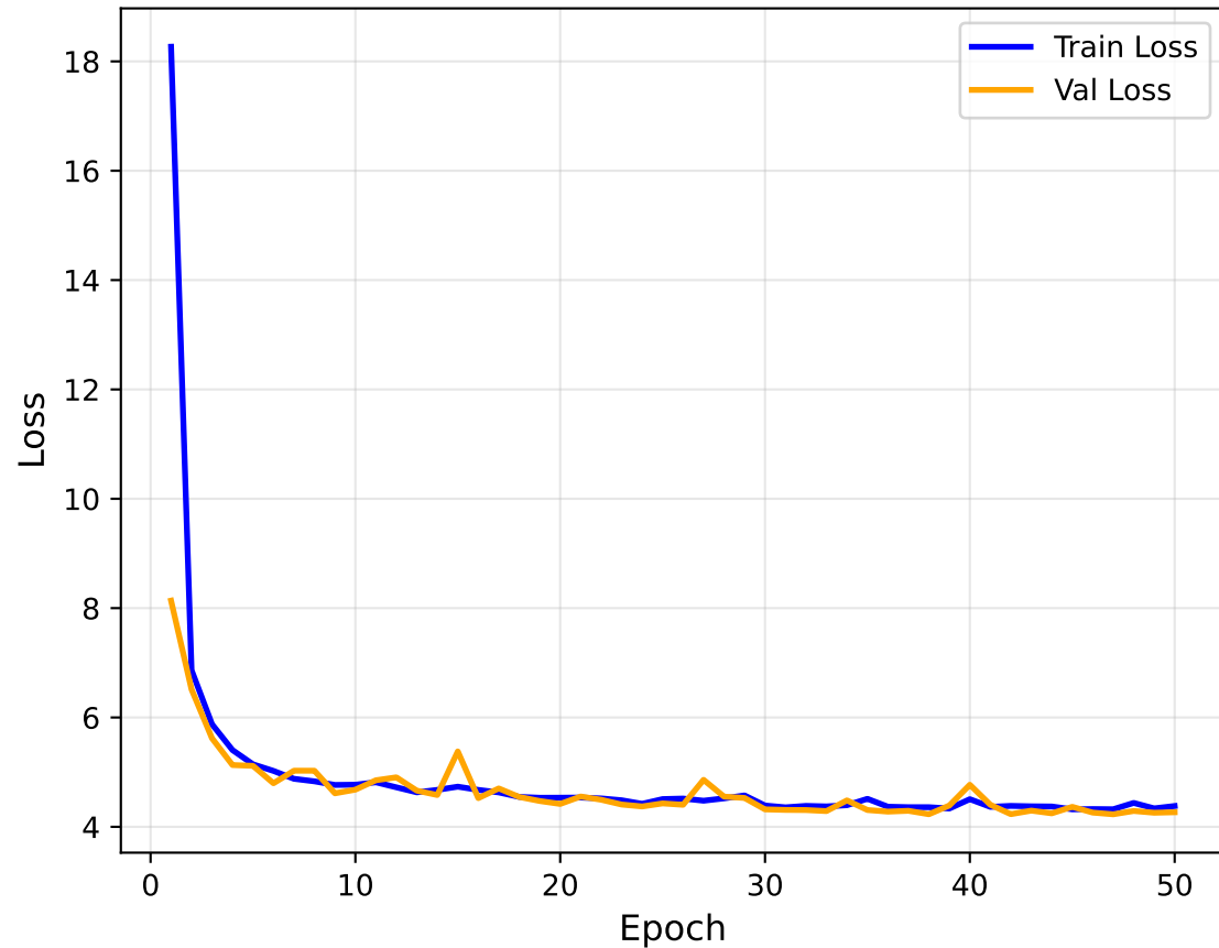
Training Curve
