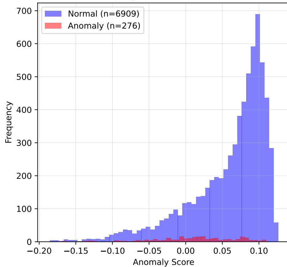
Anomaly Scores Distribution
