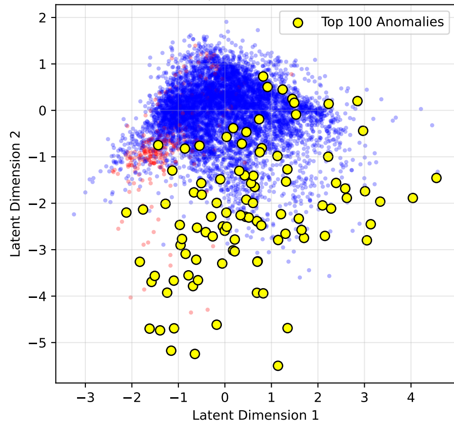
Latent Space with Anomalies
