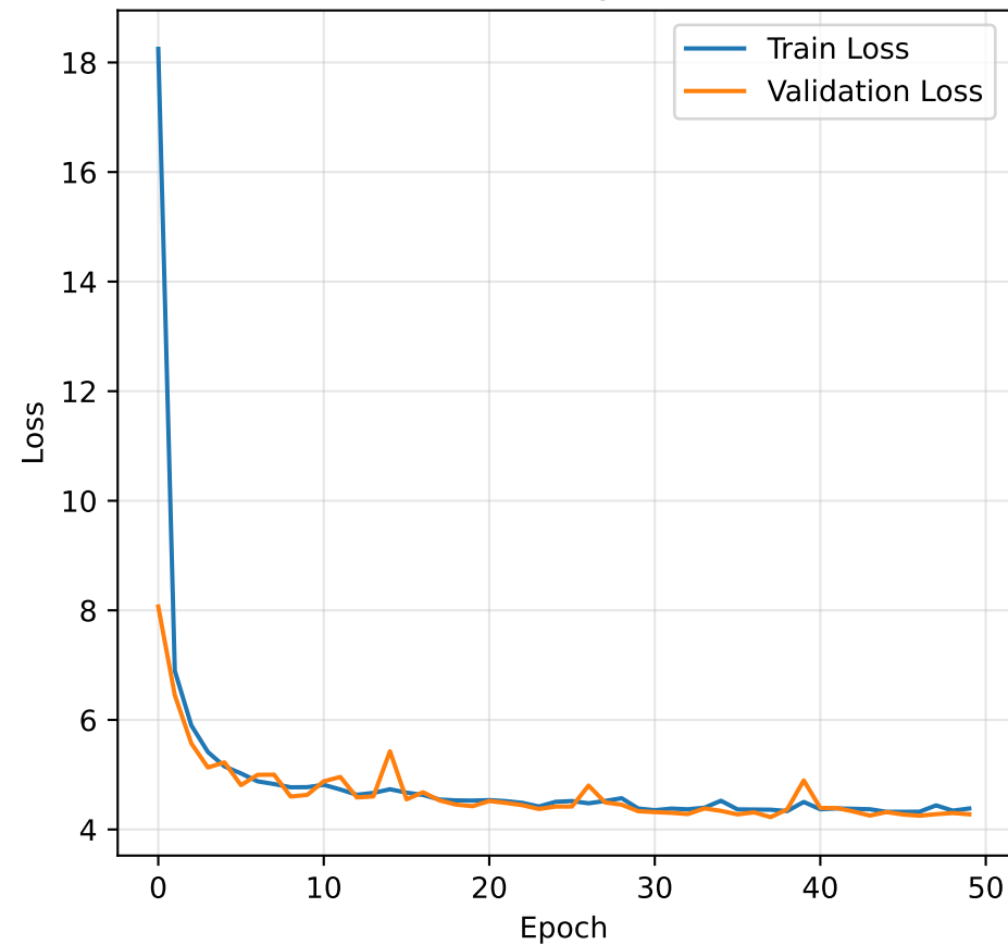
VAE Training Curve
