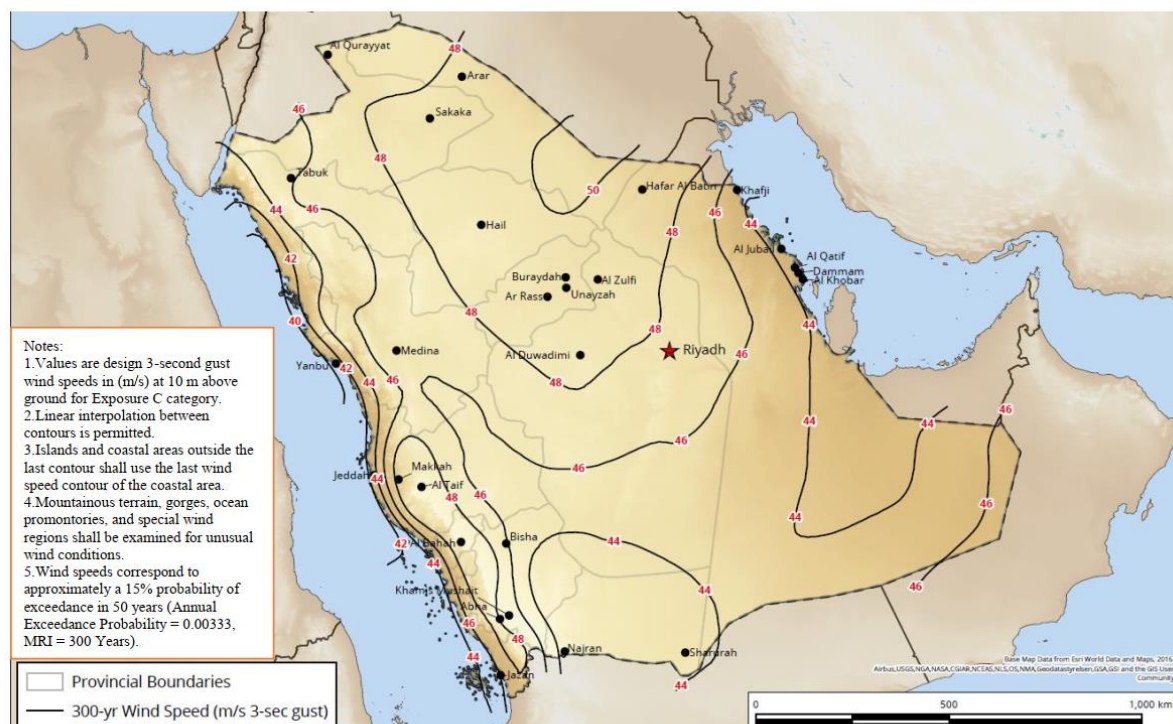
Figure 26-2C: Ultimate wind speeds for Risk Category I Buildings and other Structures.
