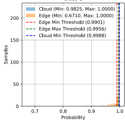
Class 5
