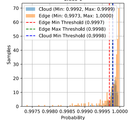
Class 9
