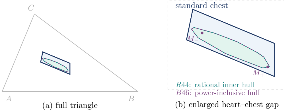
Figure 1: Actual inner-outer geometry for the diagnostic triangle A = (0, 0) , B = (21, 0) , C = (5, 12) (side lengths 13, 20, 21). The blue quadrilateral is Paper I’s standard chest. The green polygon is the rational R44 inner hull; the purple dashed boundary is the power-inclusive B46 hull for the continuous attractive class. Their difference is small at this shape, so the boundaries nearly coincide. Panel (b) magnifies the same Cartesian geometry; the two power values are marked separately.
