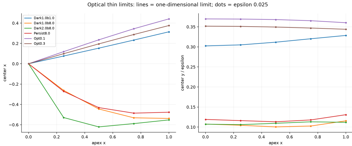
Figure 11.1: Optical thin limits: one-dimensional limiting integrals compared with finite-thickness numerical triangles. This is a cross-check of two different numerical representations, not an interval error certificate.
