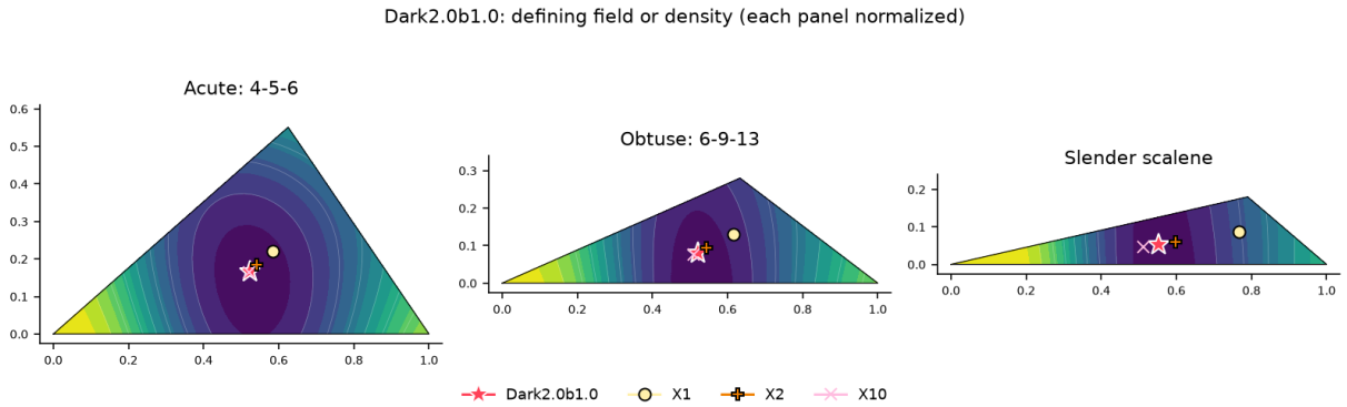
Figure 9.5: Field/density atlas in three scalene triangles. Red star: selected PITC; other markers: X(1) , X(2) , X(10) . Each panel is separately normalized; these illustrative discretizations are not error enclosures.
