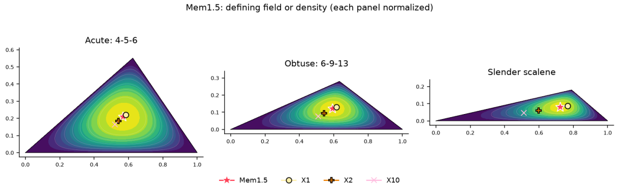
Figure 6.7: Field/density atlas in three scalene triangles. Red star: selected PITC; other markers: X(1), X(2), X(10). Each panel is separately normalized; these illustrative discretizations are not error enclosures.
