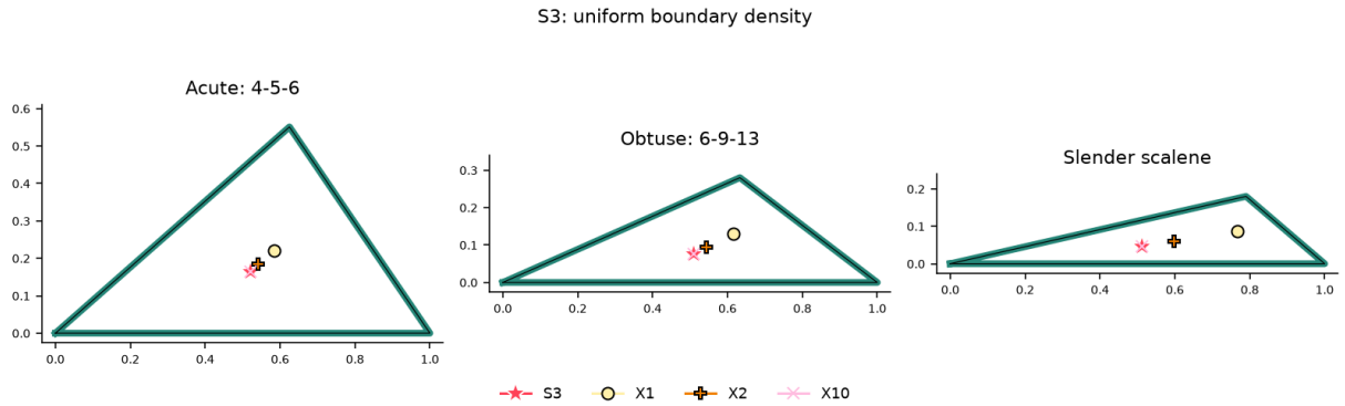
Figure 5.6: Field/density atlas in three scalene triangles. Red star: selected PITC; other markers: X(1), X(2), X(10). Each panel is separately normalized; these illustrative discretizations are not error enclosures. A boundary density replaces an interior contour plot for this boundary-supported measure.
