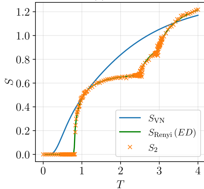
(c) Entropy
