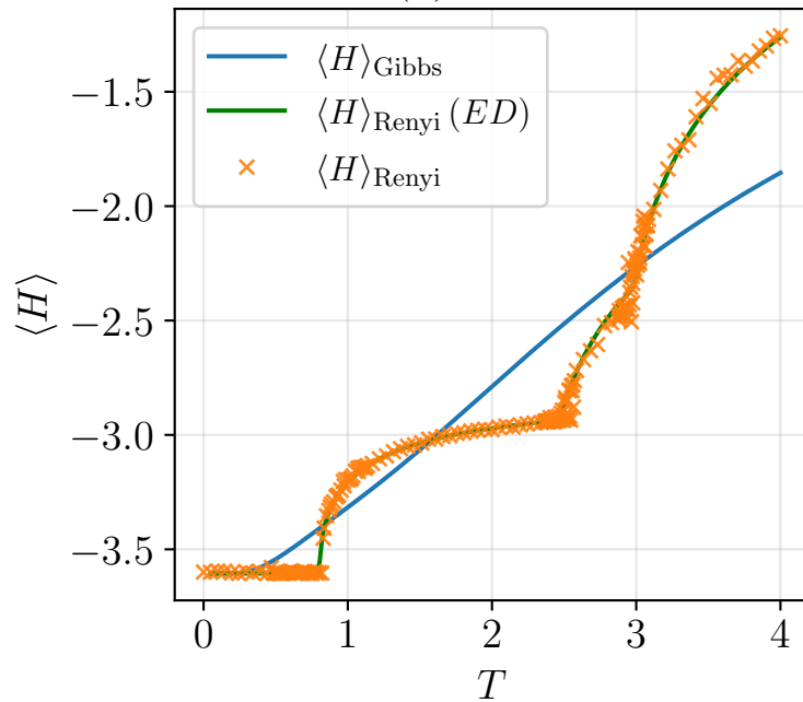
(b) Energy
