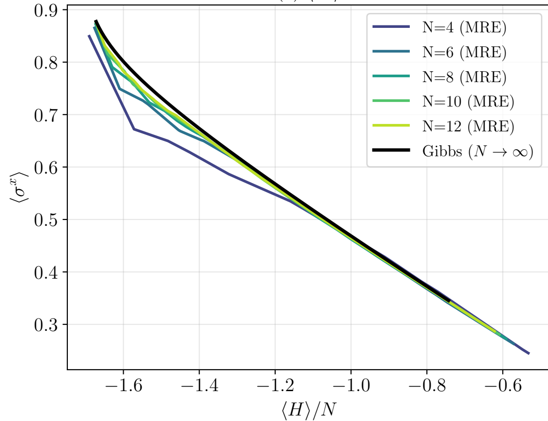
(a) \langle \sigma^x \rangle
