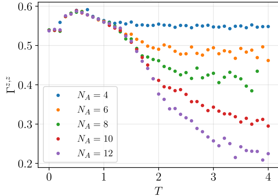
(c) \Gamma^{z,z}
