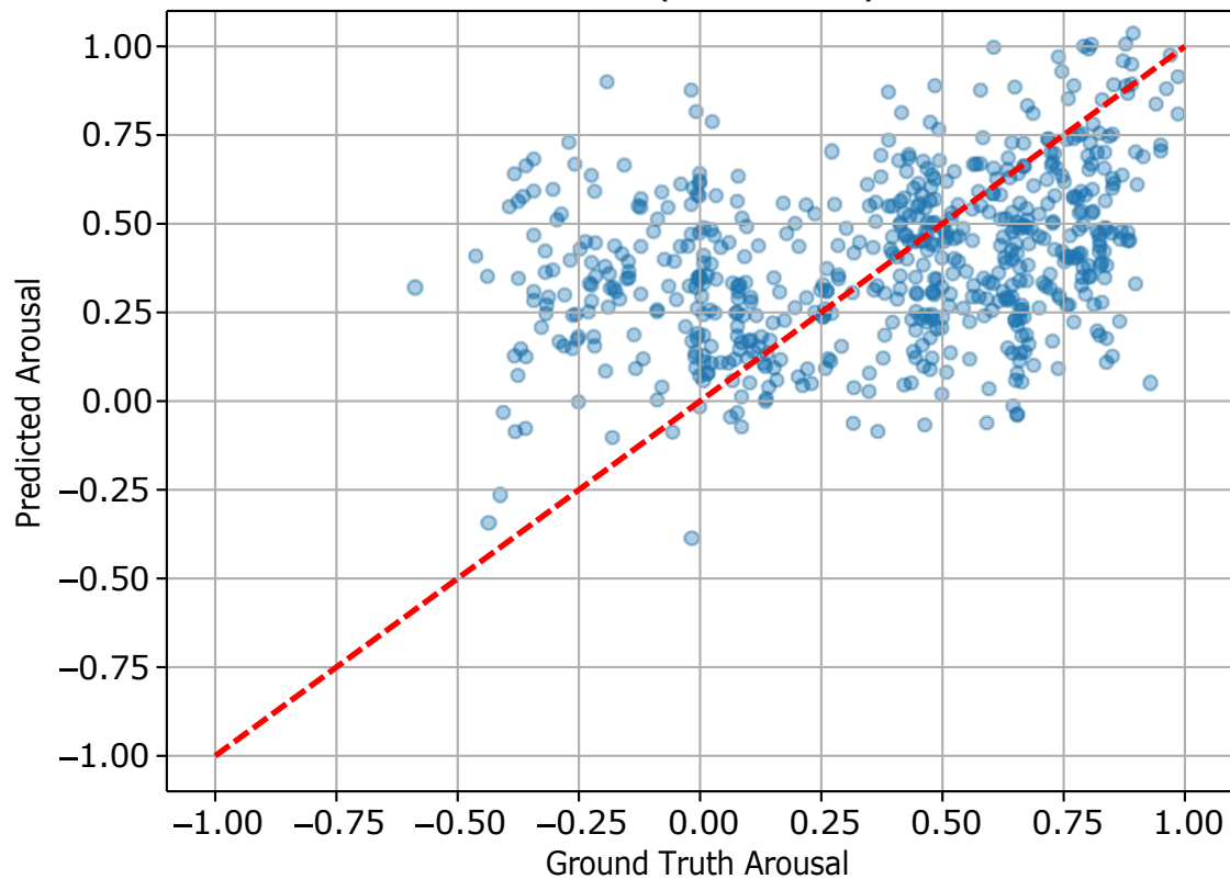
Arousal (CCC: 0.316)
