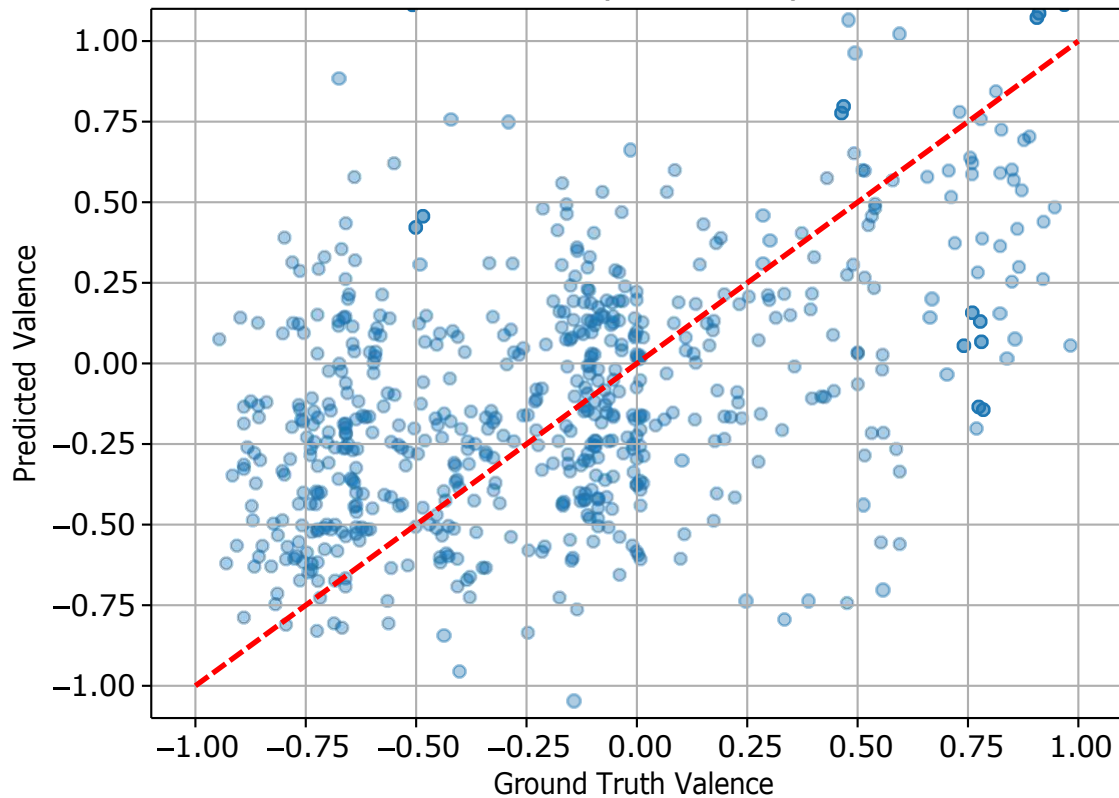
Valence (CCC: 0.464)
