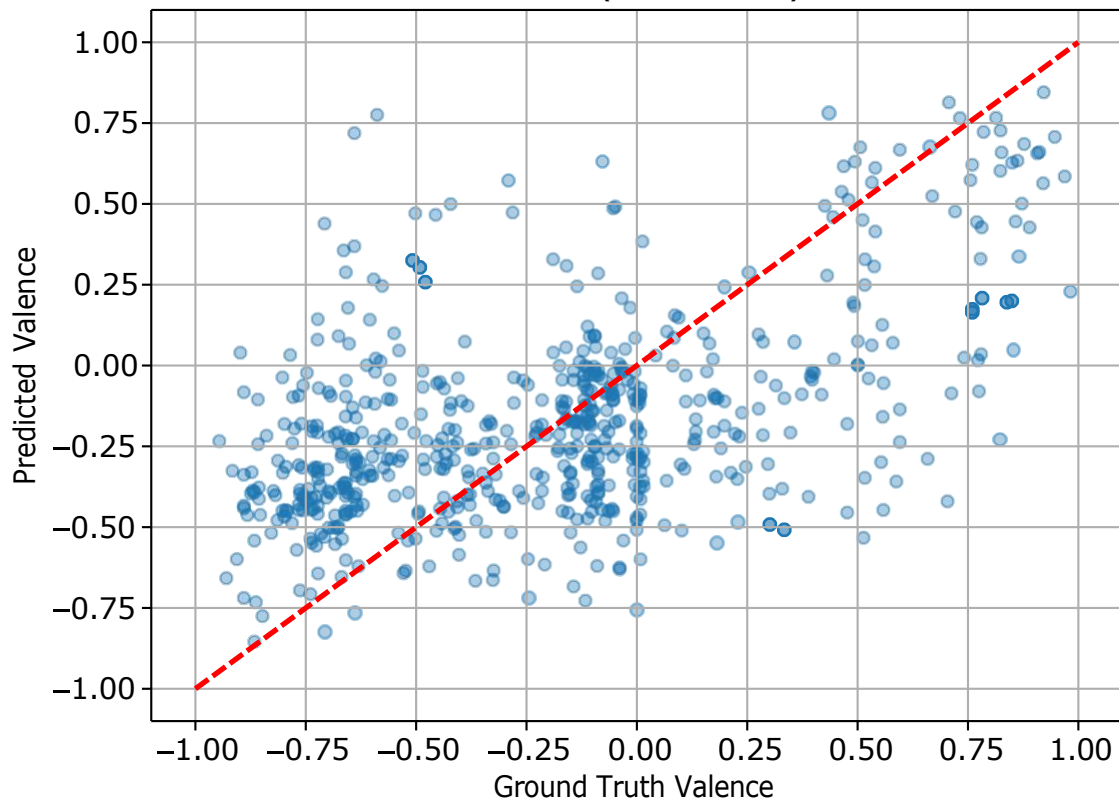
Valence (CCC: 0.498)
