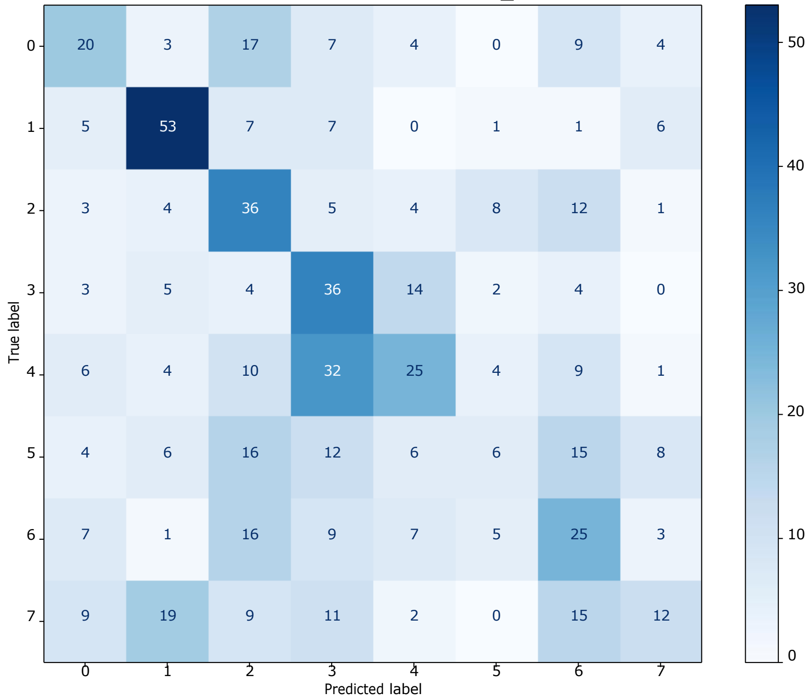
Confusion Matrix - mobilenet_v2
