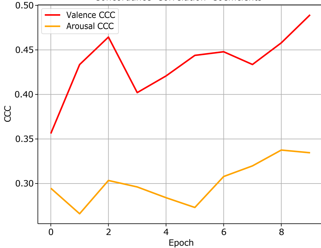
Concordance Correlation Coefficients
