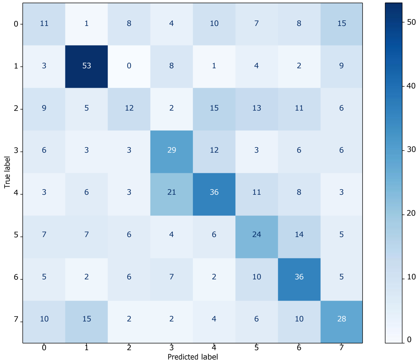
Confusion Matrix - resnet18
