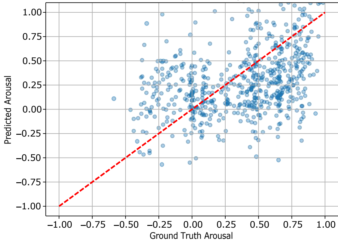
Arousal (CCC: 0.394)
