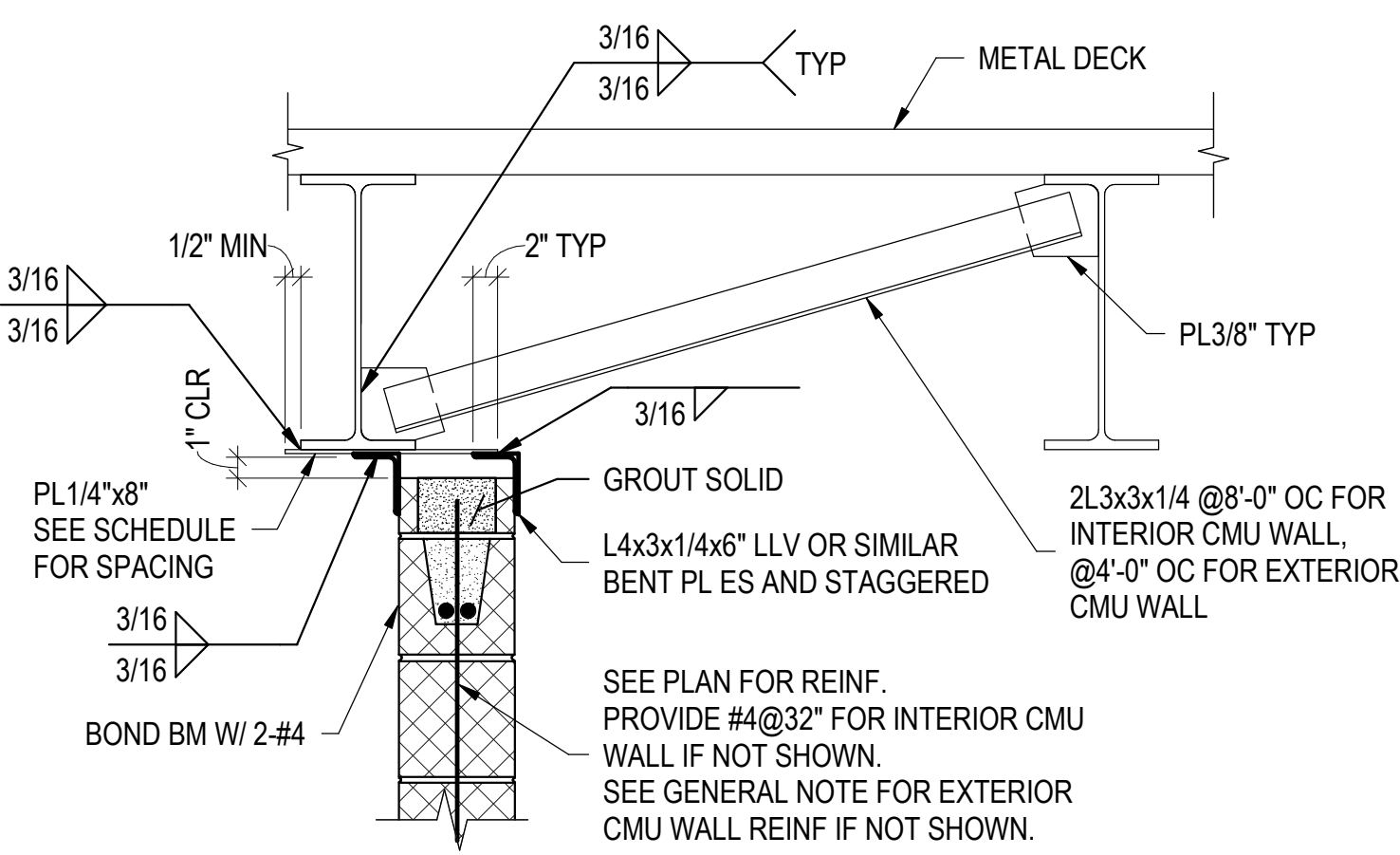
TYPICAL CMU WALL BRACING UNDER ROOF DECK DETAIL
