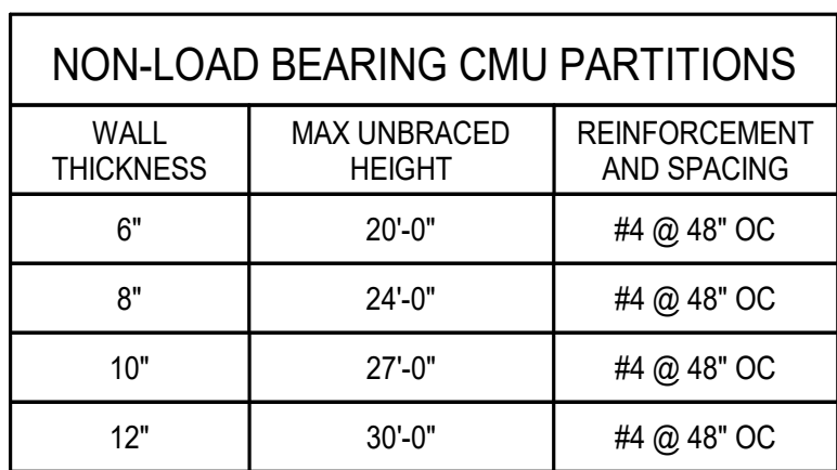
TYPICAL INTERIOR CMU WALL REBAR SCHEDULE
