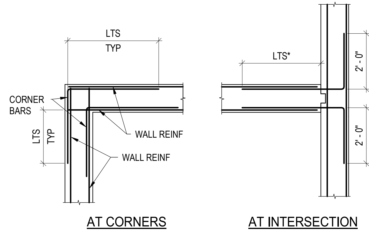
TYPICAL HORIZONTAL WALL REINF DETAIL
