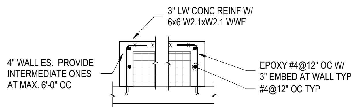
6" EPOXY #4 @ 12" OC W/ 3" EMBED AT WALL 3" LW CONC REINF W/ 6x6 W2.1xW2.1 WWF ARDEX INSULATION, SEE GEN NOTES BASE SLAB 3" MAX
