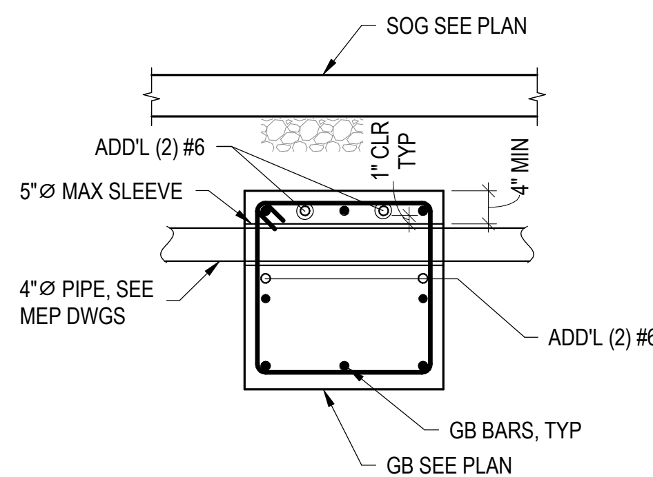
TYPICAL SLEEVE PENETRATION DETAIL AT GRADE BEAM
