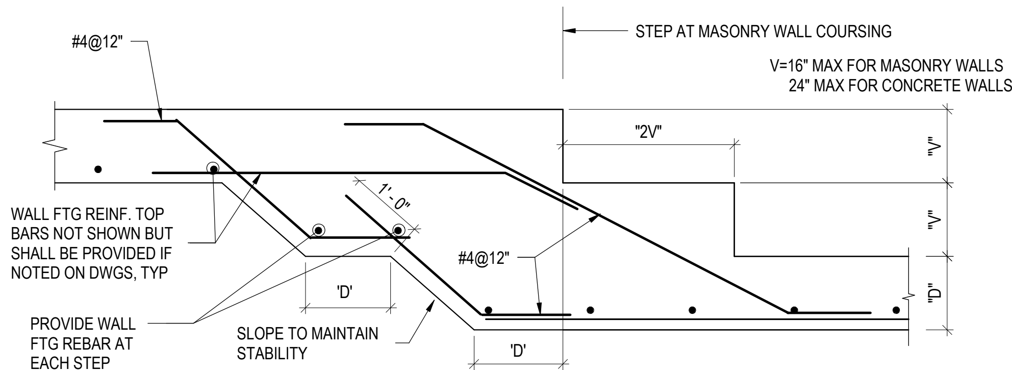
TYPICAL STEPPED FOOTING DETAIL
