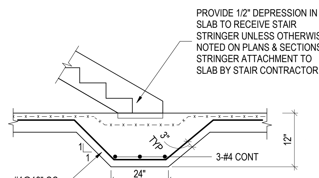
TYPICAL THICKENED SLAB ON GRADE DETAIL
