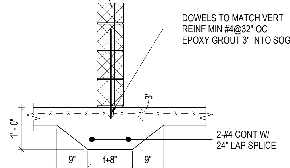
TYPICAL NON-LOAD BEARING CMU ON SLAB ON GRADE DETAIL
