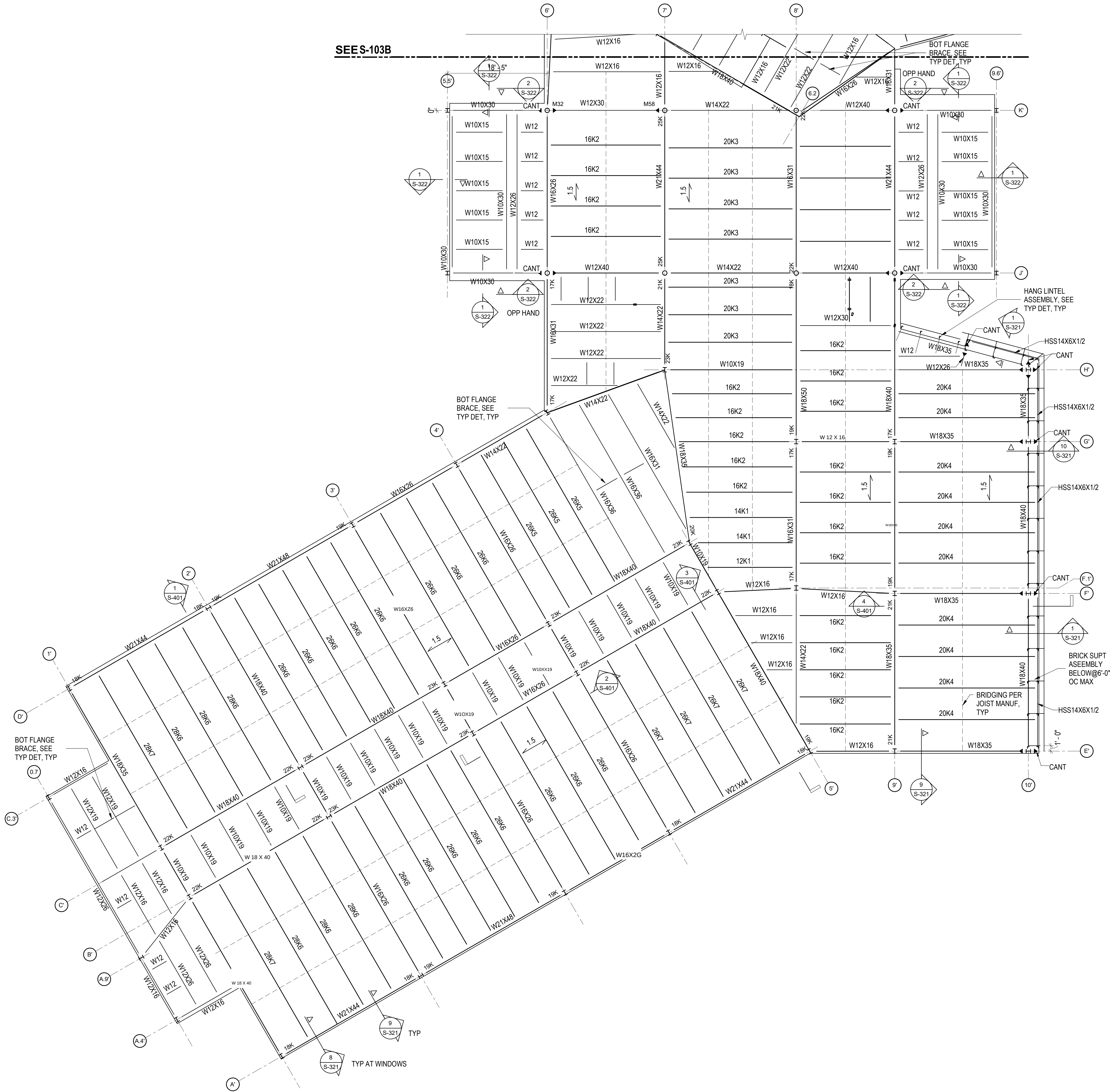
1 MAIN ROOF FRAMING PLAN - PART A 1/8" = 1'-0"
