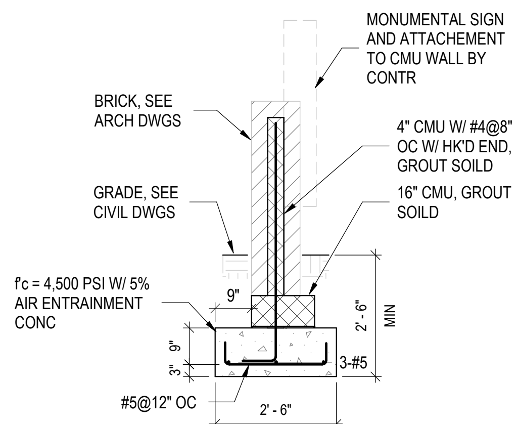
MONUMENTAL SIGN DETAIL
