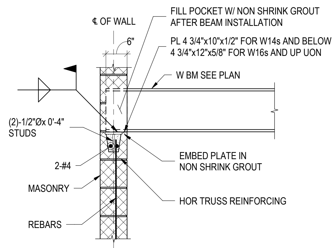
TYPICAL STEEL BEAM BEARING ON MASONRY
