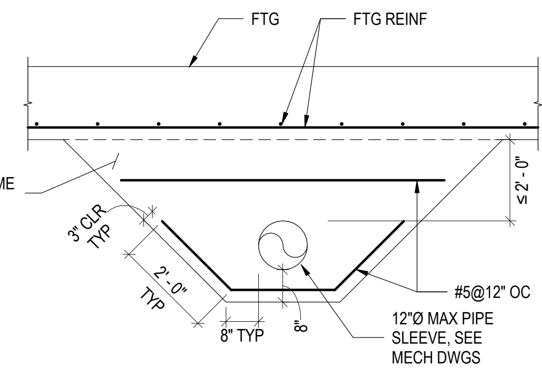
TYPICAL PIPE UNDER FOOTING DETAIL
