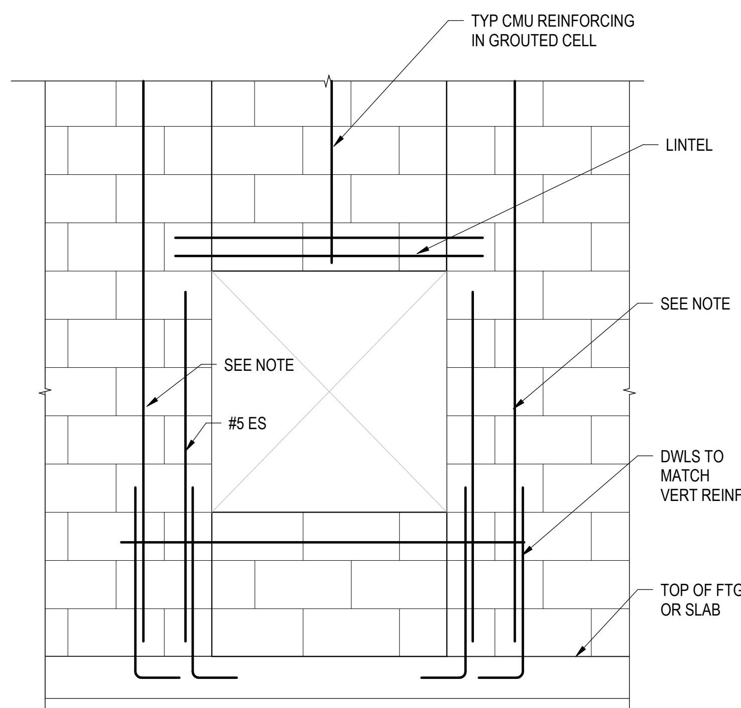
TYPICAL WALL REINFORCING AT CMU WALL OPNG DETAIL
