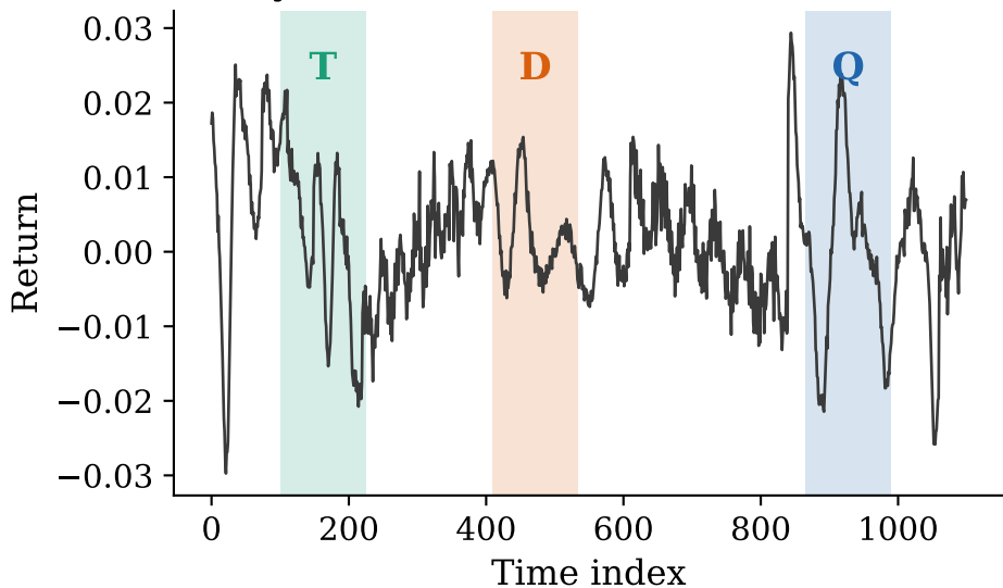
(A) Synthetic series with selected windows
