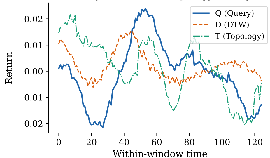
(B) Query vs DTW and topology analogues
