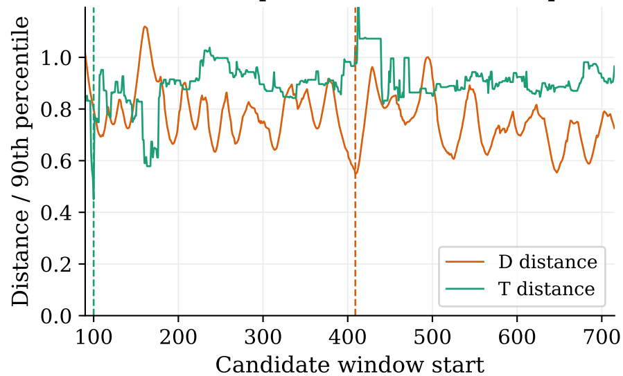
(C) Distance profiles over candidate pool
