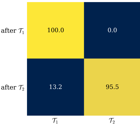
(c) Replay
