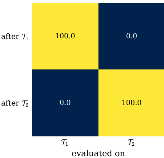
(c) LwF
