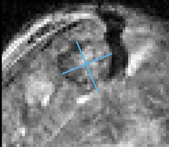
RECIST crosshair
