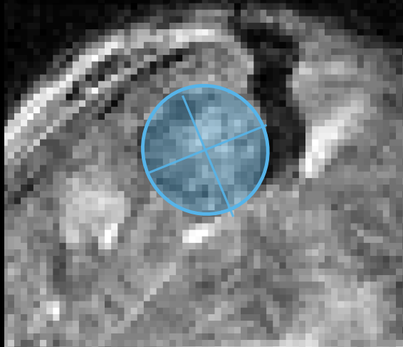
Fitted ellipse
