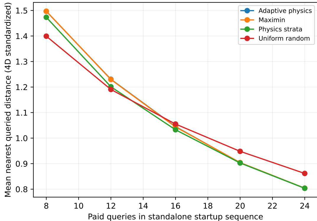
NEW-136 development: class discovery and geometric coverage
