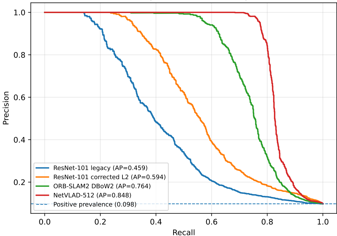
KITTI-05 test precision--recall comparison
