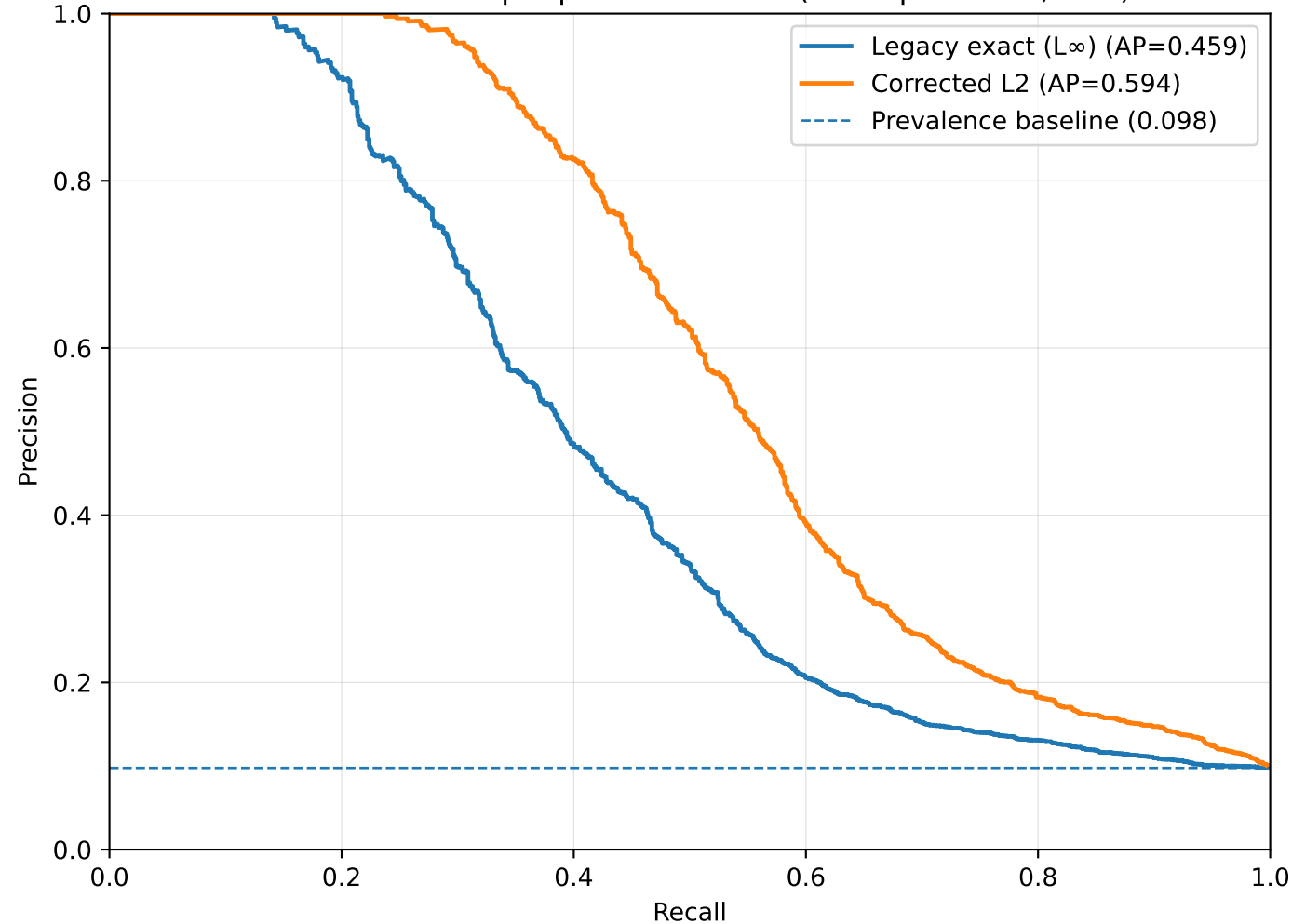
KITTI 05 — Test split precision-recall (descriptor level, L=1)
