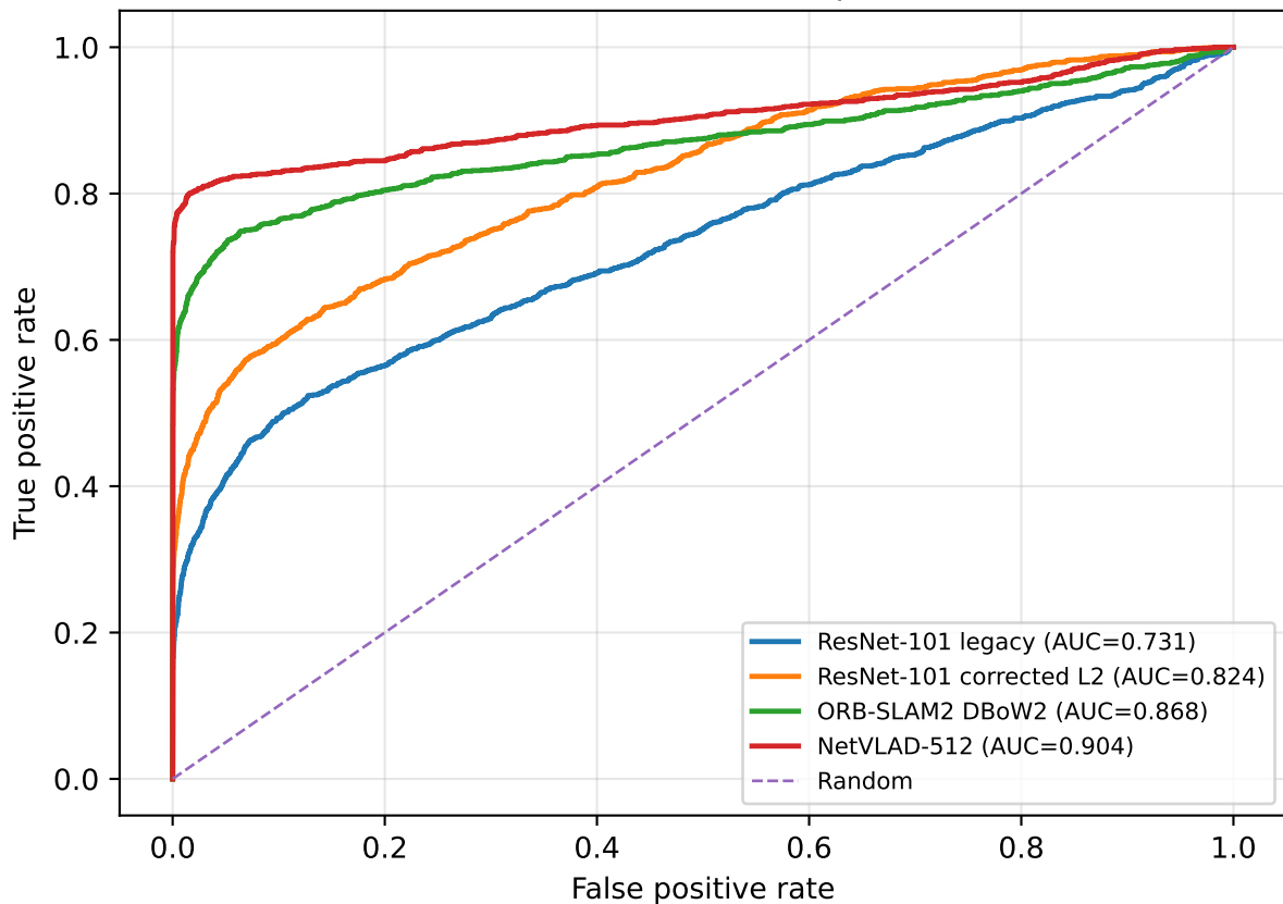
KITTI-05 test ROC comparison
