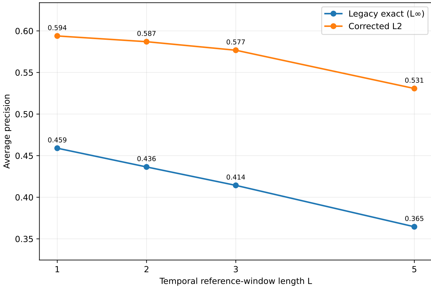
KITTI 05 — Temporal ablation on the held-out test event
