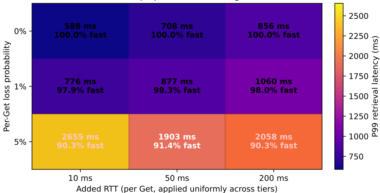
LBVR-Med fast-path P99 — WAN conditions matrix (50 bundles × 30 reps per cell; SLO budget = 2000 ms)
